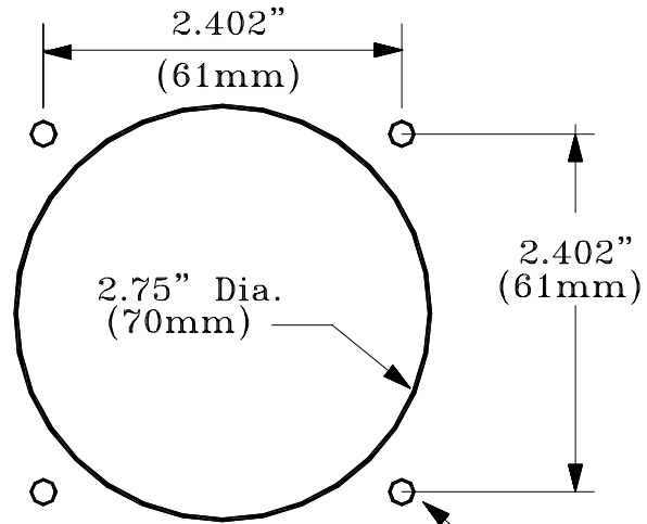
PANEL MOUNTING OPTION #1
