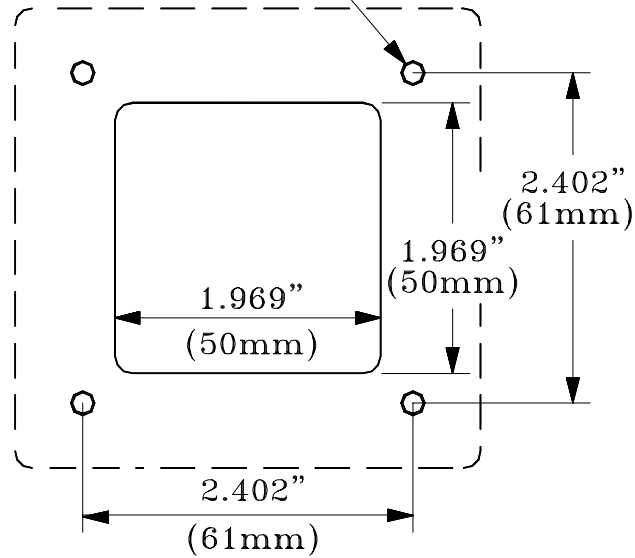
PANEL MOUNTING OPTION #2
